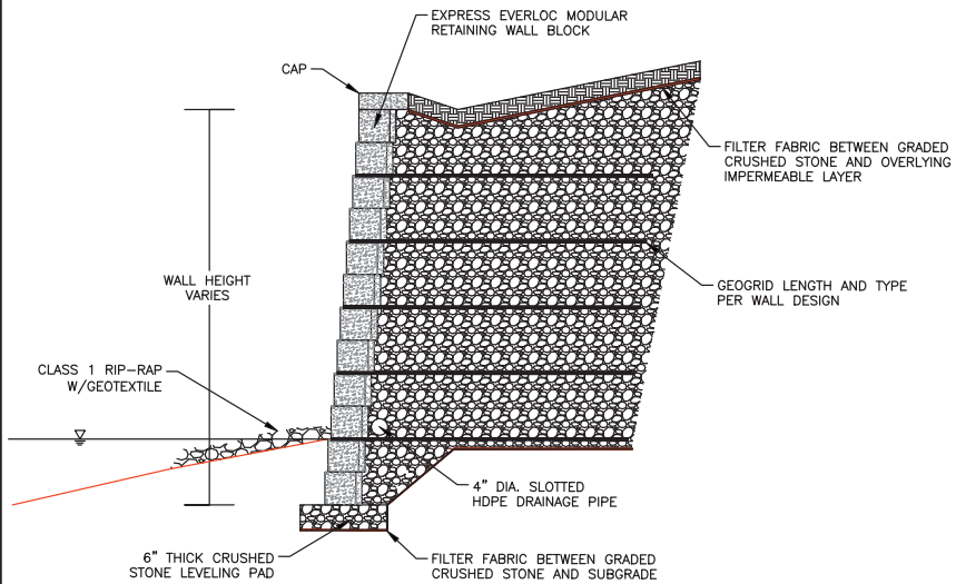
TYPICAL SHORELINE PROTECTION DETAIL N.T.S.
