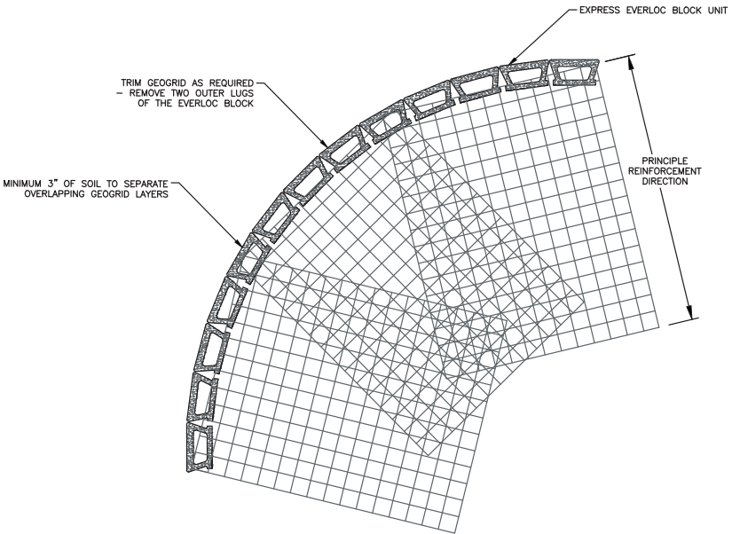
TYPICAL OUTSIDE RADIUS DETAIL N.T.S.
