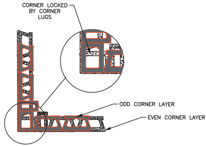
EXPRESS CORNER ASSEMBLY DETAIL N.T.S.
