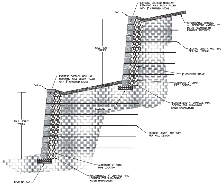
EXPRESS TIERED WALL DETAIL N.T.S.
