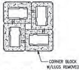
FOUR UNIT - LEFT-END COLUMN DETAIL
