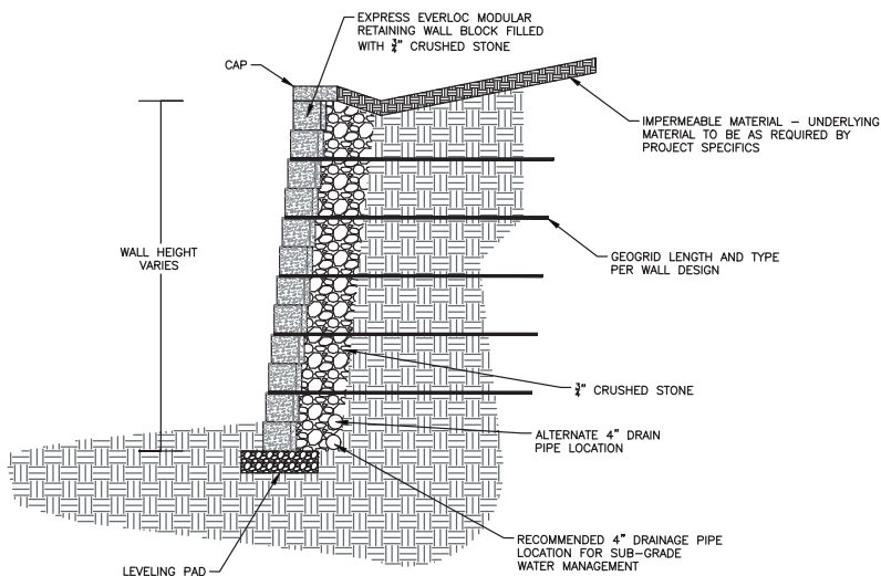
EXPRESS RETAINING WALL DESIGN N.T.S.
