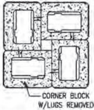
FOUR UNIT - RIGHT-END COLUMN DETAIL
