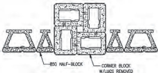
FOUR UNIT - LEFT-END COLUMN DETAIL SECOND ROW - W/SETBACK
