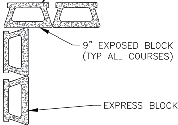
EXPRESS EVEN CORNER DETAIL N.T.S.
