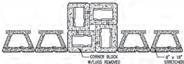
FOUR UNIT - RIGHT-END COLUMN DETAIL FIRST ROW
