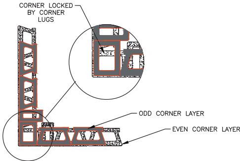
EXPRESS CORNER ASSEMBLY DETAIL N.T.S.
