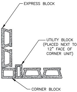
EXPRESS EVEN CORNER DETAIL N.T.S.
